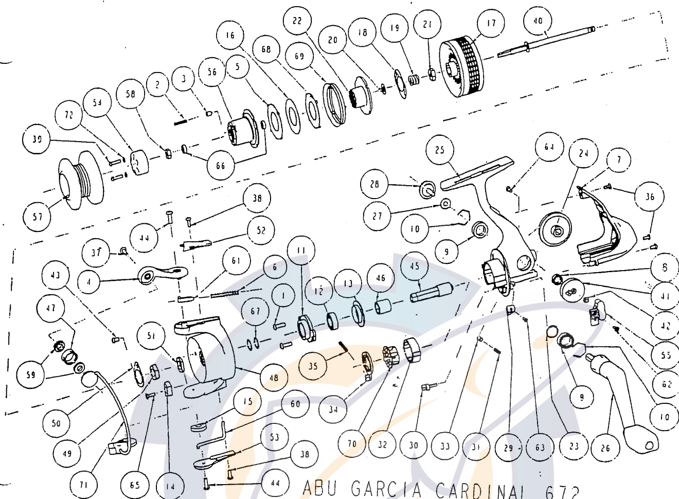
Abu Garcia Cardinal 672 Parts List
